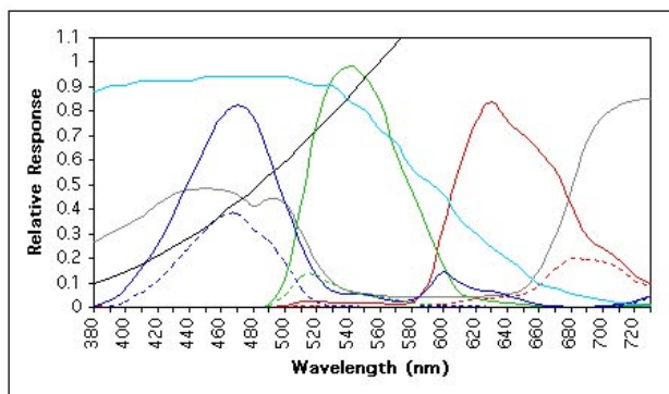
Figure 15a. Tungsten illumination (—) combined with the reflectance of cobalt blue (—), a daylight filter (—), the silicon sensor RGB responses (—, —, —) and the results (- - -, - - -, - - -).
