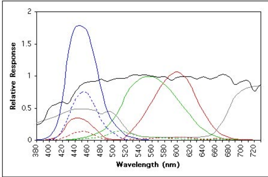
Figure 12. D-50 illumination (—) combined with the reflectance of cobalt blue (—), the CIE 1931 standard observer (—, —, —) and the results (---, ---, ---).
