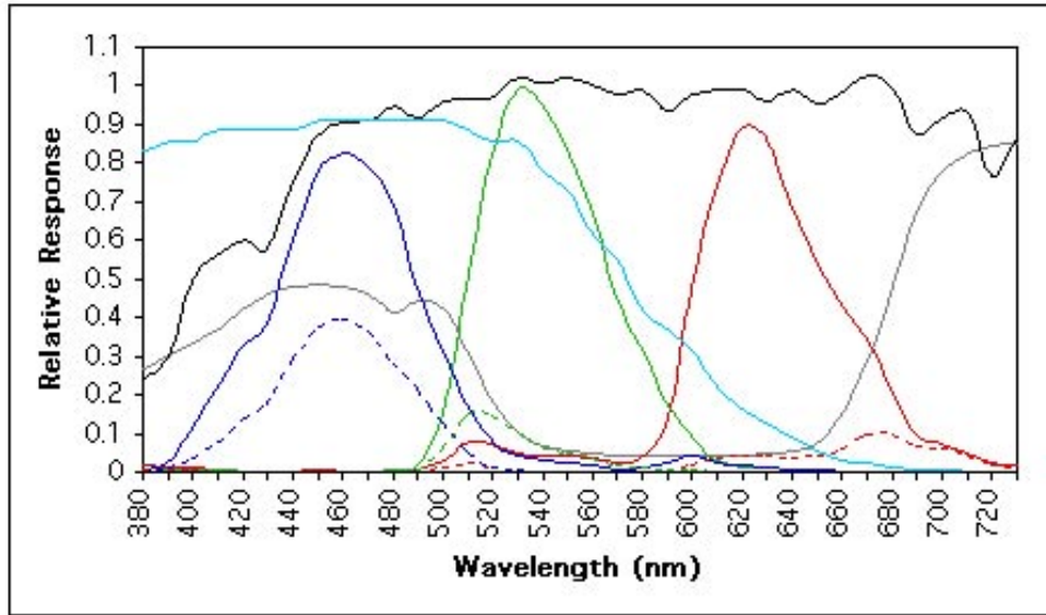
Figure 14. D-50 illumination (—) combined with the reflectance of cobalt blue (—), a tungsten filter (—), the silicon sensor RGB responses (—, —, —) and the results (---, ---, ---).
