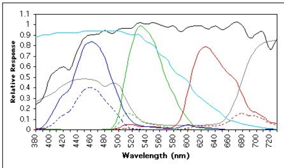
Figure 13. D-50 illumination (—) combined with the reflectance of cobalt blue (—), a daylight filter (—), the silicon sensor RGB responses (—, —, —) and the results (---, ---, ---).
